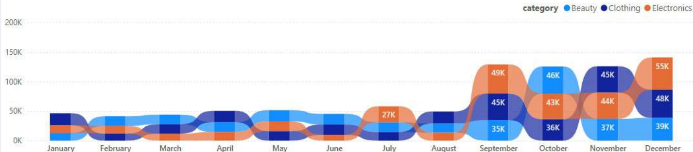
Seasonal Pattern
